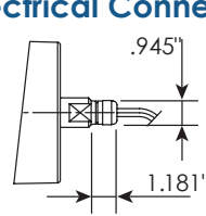
Straight brass connector with 1.5m cable (longer cable lengths available)
