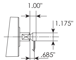
Stainless Steel elbow connector with 1.5m cable (longer cable lengths available)
